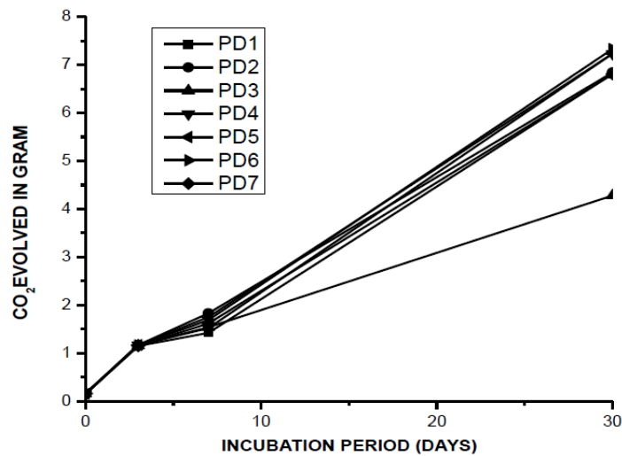
Figure 2: CO 2 evolution during biodegradation of polyethylene.
